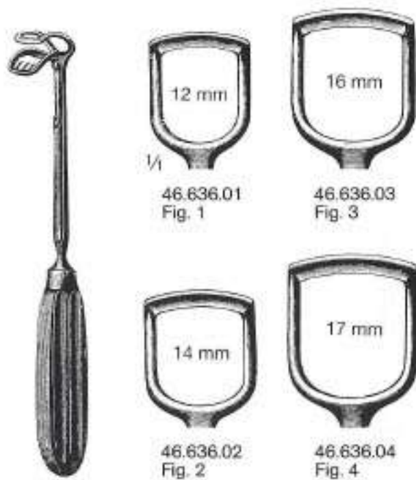
St. CLAIR-THOMSON 46.636.01-46.636.04 21 cm
